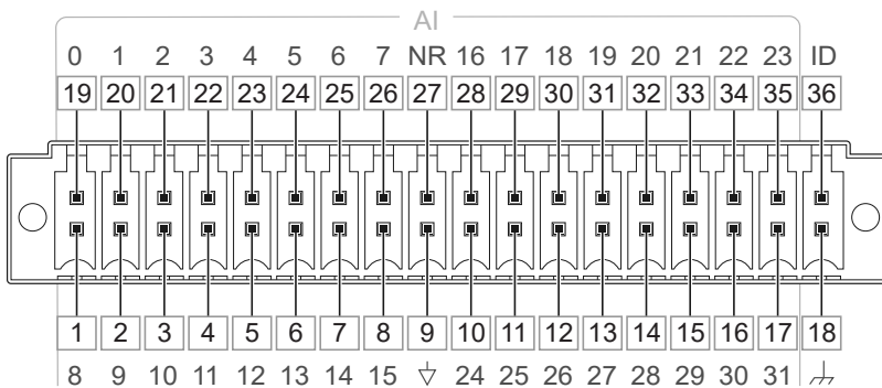
Figure 1. USB-6423 AI Connector Pinout
